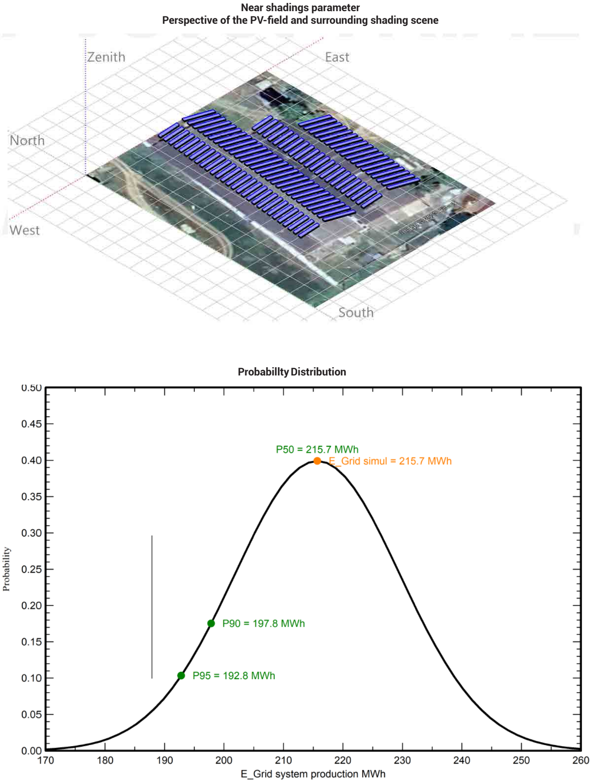
Figure 8: RTPV assessment on industrial building in Rajapalayam LPA and estimated energy generation
